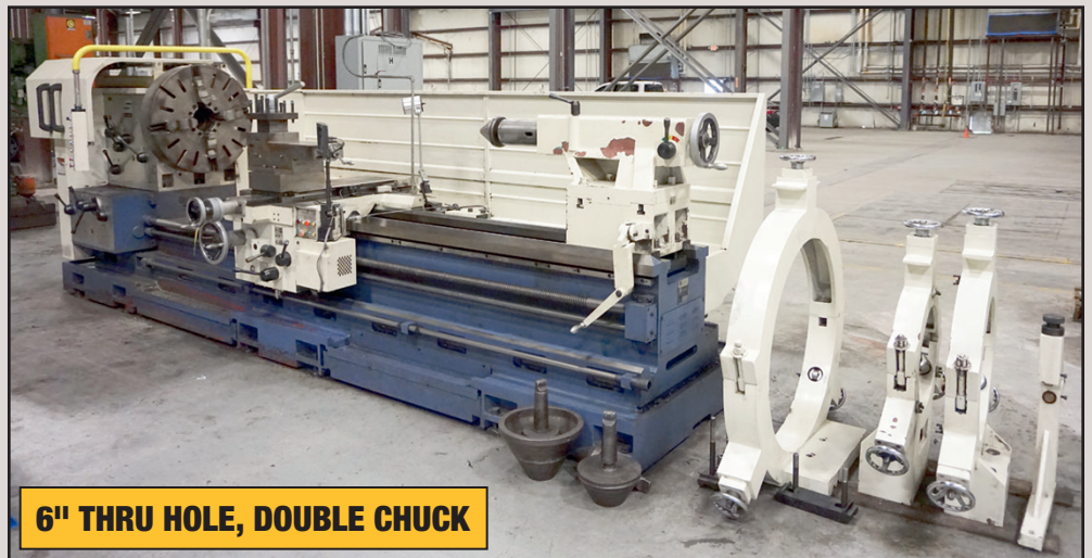
SUMMIT 42-6X120 LATHE, W/3 STEADY REST, 1 FOLLOW REST, 3 LIVE CENTERS TAILSTOCK W/NEWELL DRO, 31" 4-JAW CHUCK, 10' BED
